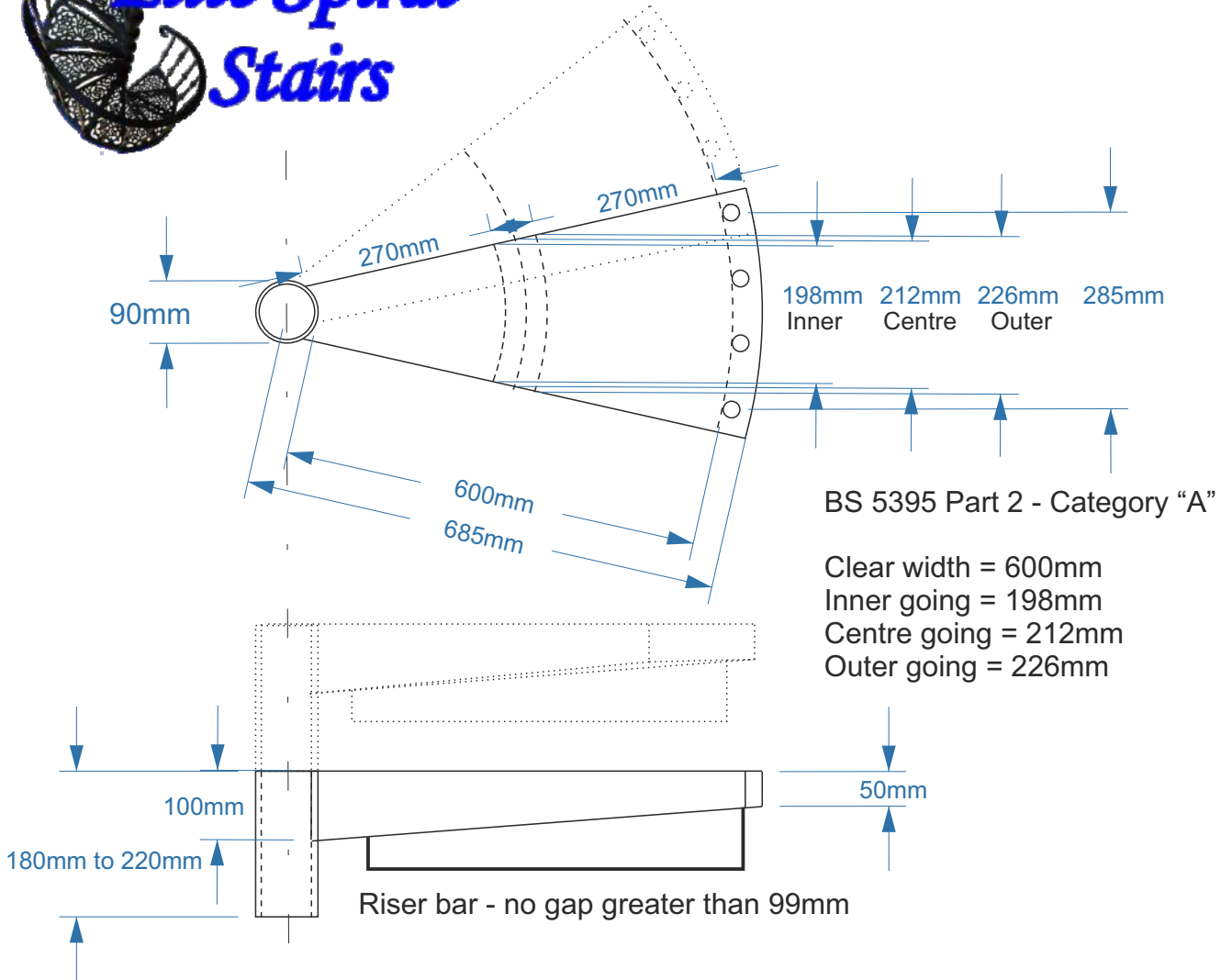
1400mm diameter Spiral Stair Fire escape tread : Scale - 1:10
